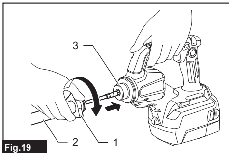
Fig.19 ► 1. Cople 2. Entubado exterior 3. Rosca macho
